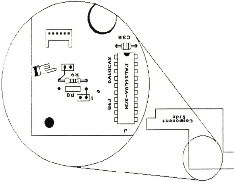
Figure 5: Detail of WCS board, showing PAL and jumper locations
